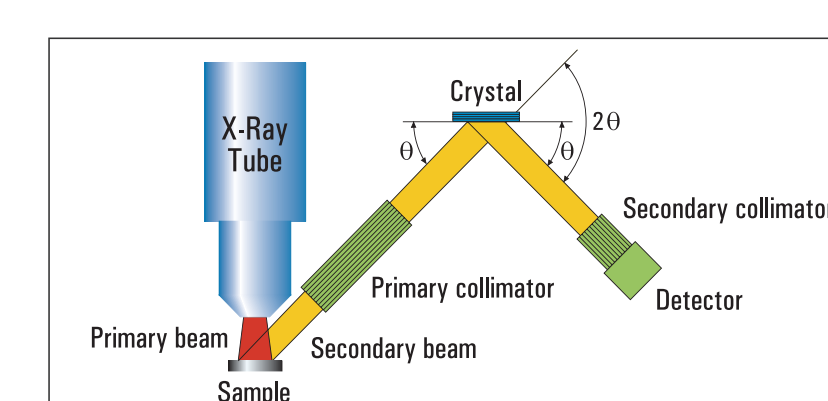
The Flat Crystal Spectrometer
