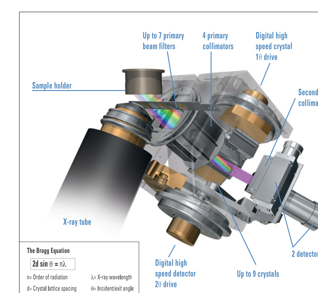
Exclusive Gearless Goniometer Principle of Operation
