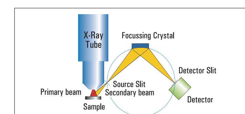
The Focusing Crystal Spectrometer
